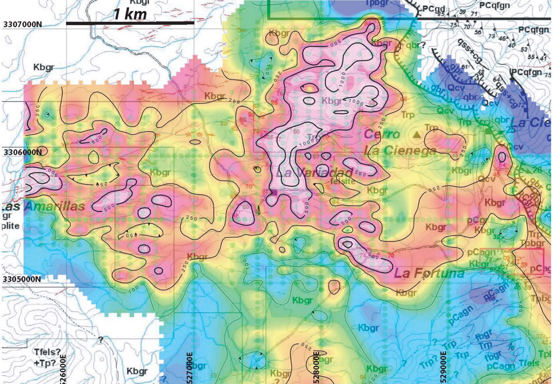
Anomalous Copper in Soils: Northern Leon Property (contours in ppm Copper)
