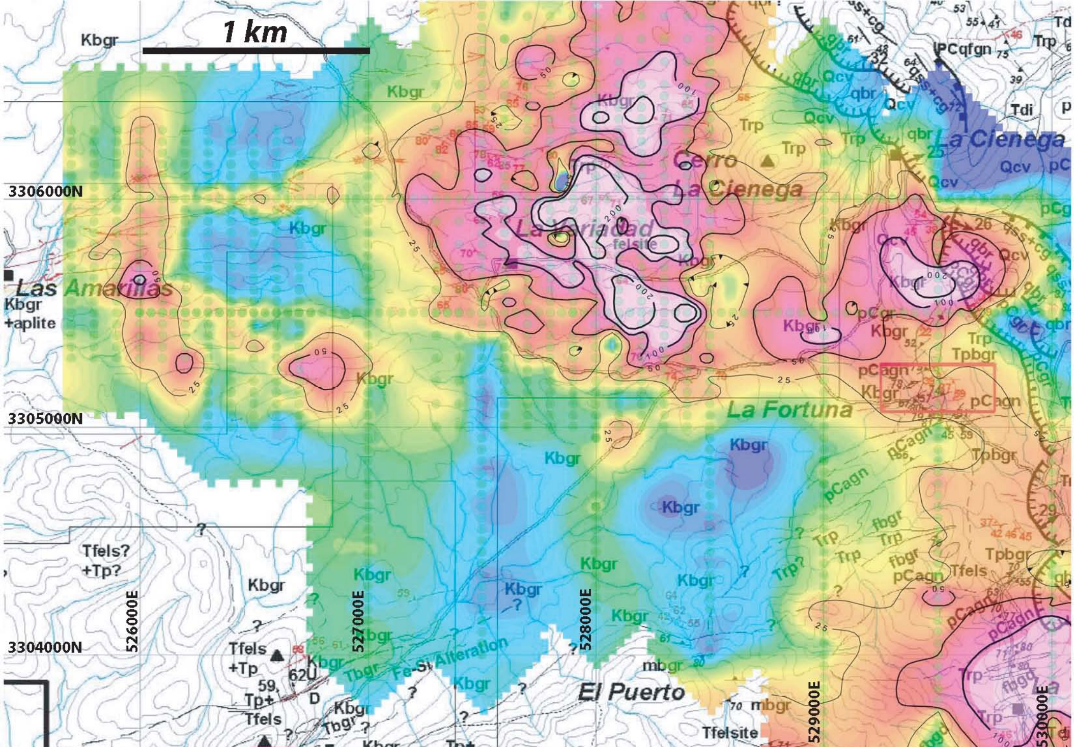
Anomalous Molybdenum in Soils: Northern Leon Property (contours in ppm Molybdenum)
